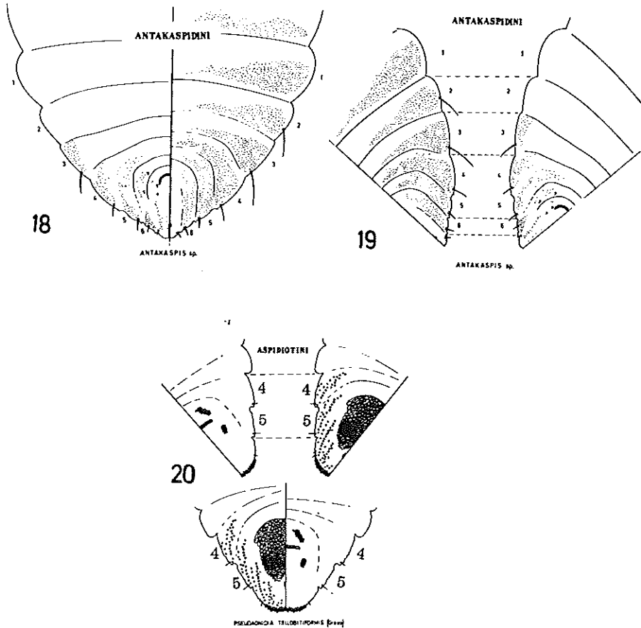
Figs. 18-19. Antakaspis sp. Schematic drawings of ventral and dorsal aspects of adult female. Fig. 20. Pseudaonidia trilobitiformis (Green), Schematic drawings of ventral and dorsal aspects of adult female.
