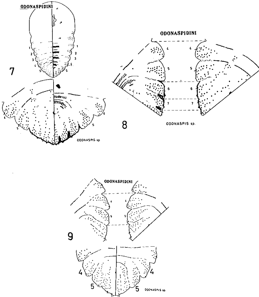
Figs. 7-9. Odonaspis sp. Schematic drawings of ventral and dorsal aspects, 7-8. Adult female. 9. Female second instar.
