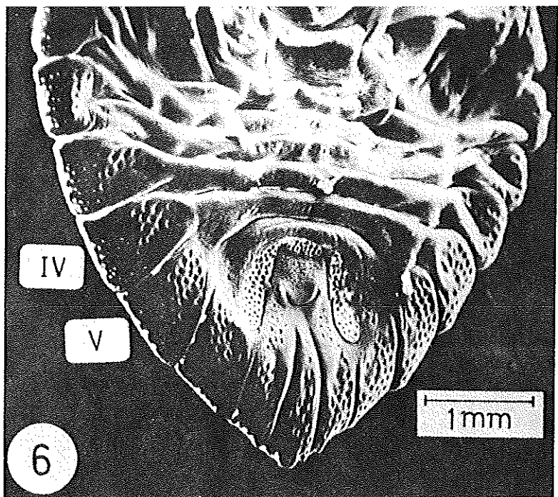
Figs. 5-6. Odonaspis ruthae Kotinsky, adult female. 5. Photograph of tergites and sternites of fourth and fifth abdominal segments (Intersegmental sutures slightly retouched). 6. Micrograph of ventral aspect of abdominal segments.
