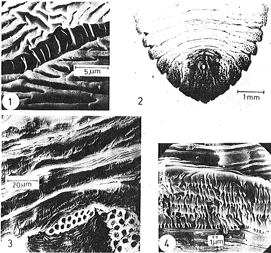
Figs. 1-4. Odonaspis spp. Adult females. 1. Micrograph of intersegmental suture with spicules. 2. Photograph of abdominal segments in slide-mounted specimen. 3-4. Micrographs of ventral crenulae.
